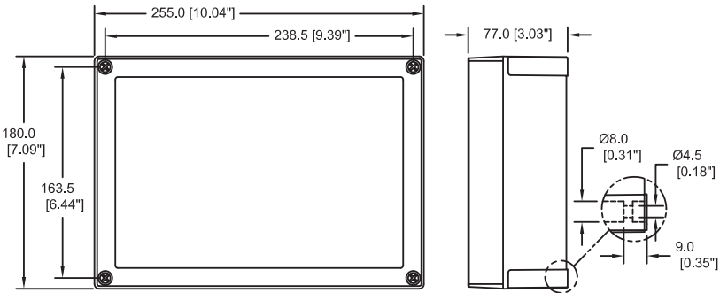
Non-ATEX Approved Polycarbonate Enclosure
